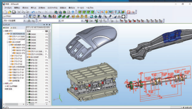
View function
